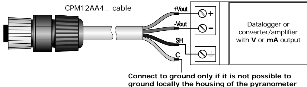
Fig. 4.1: LPPYRA03 connections
